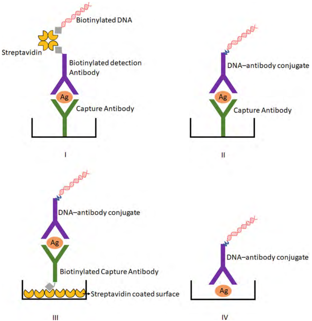
Fig. 1 Schematic diagram of the various Immuno-qPCR assay formats presented here. (I) The capture antibody is first adsorbed to the PCR tube surface, and streptavidin is used to couple biotinylated DNA to biotinylated detection antibody. (II) The capture antibody is first adsorbed to the PCR tube surface, and a DNA-antibody conjugate is mixed with the antigen or sample before addition to the well. (III) Streptavidin-coated microtiter plates are used, and biotinylated capture antibody, DNA-antibody conjugate, and antigen or sample are pre-mixed before addition to the well. (IV) Antigen and samples are adsorbed to the surface of the well prior to the addition of DNA-antibody conjugate
