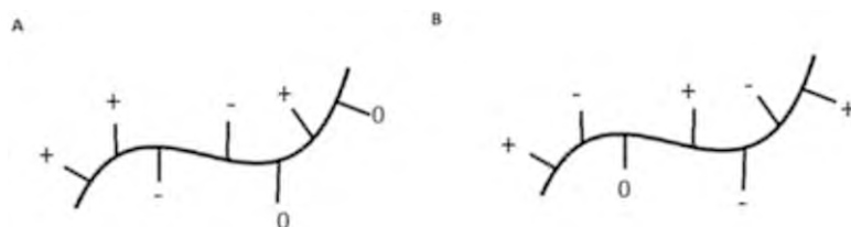
Fig. 1 A section of a protein with positively and negatively charged amino acid side chains. (a) Protein with more positive than negative charges which will make the protein positively charged overall (note the side chain with 0 charge). (b) The positive and negative charges equally balanced (isoelectric point)
