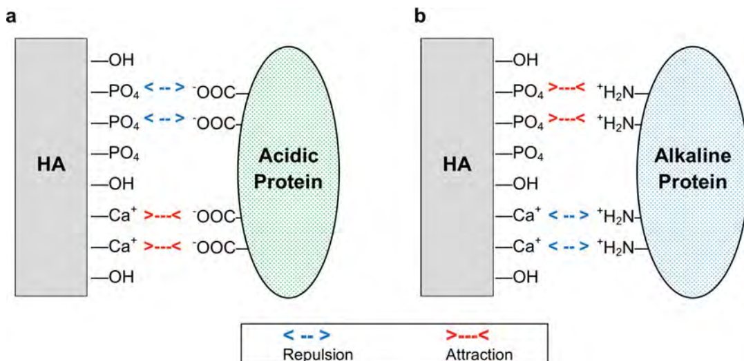
Fig. 1 Schematic representation of protein interaction with HA. (a) The carboxyl clusters on acidic proteins are repelled (electrostatically) by PO 4 groups on HA. However, the carboxyl groups form metal coordination complexes with Ca + on the HA at acidic and neutral pH. (b) Alkaline proteins form ionic bonds between PO 4 and amino groups. However, there is also simultaneous repulsion between Ca + and amino groups
